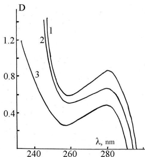
Fig.5. UV absorption spectra of water with the addition of an inhibitor ( \tau = 72 h) after 1 hour of extraction, ml/l: 1-50, 2-100, 3-150
